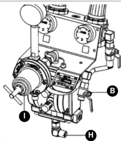
I) Paint Pressure Regulator B) 2-way Valve for Paint Recirculation H) Paint Inlet Joint
