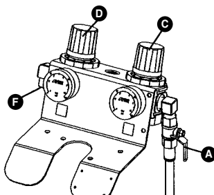
F) Air Connection to Gun D) Gun Air Pressure Reducer C) Pump Air Pressure Reducer A) Exhaust Ball Valve
